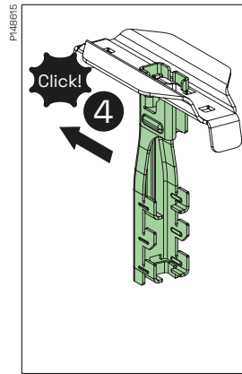
2 Press the pieces together and 3 slide the adaptor until the click lip of the adaptor pass over the locking lip of the central suspension bracket with a 4 click.
