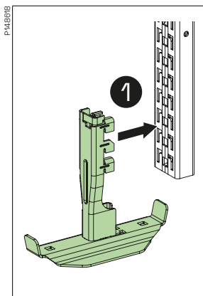
1 Push the central suspension piece until the hooks are fully inserted in the pattern and the surface touches the rail.
