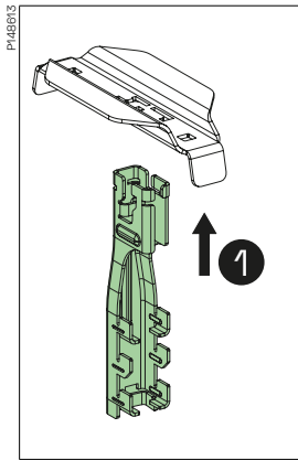
1 Insert the adaptor in the pattern on the central suspension bracket.
