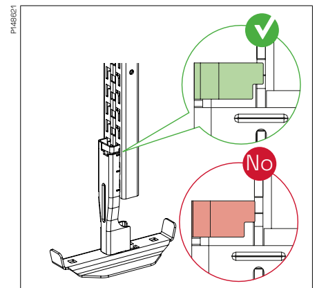
Visually check and secure that the adaptor is properly positioned, and the click lip is properly positioned inside of the slot of the CLX 3 rail.
