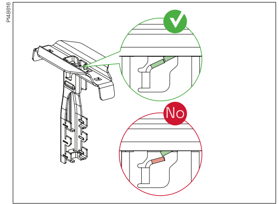
Visually check and secure that the adaptor is properly positioned, and the click lip has overpassed the locking lip.
