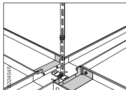
Suspension with Pendant strip W33.
