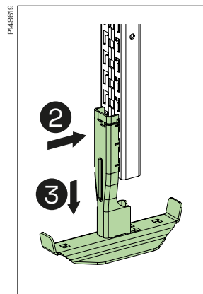
2 Press towards the rail and 3 pull down until the click lip.
