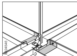
Suspension with Pendant rail W32 and half a Pendant attachment W21.
