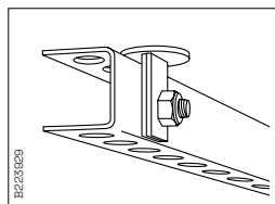
Mounting of holed beam.
