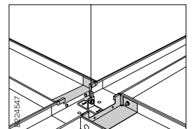
Suspension with wire and Ogebe fixing type E.
