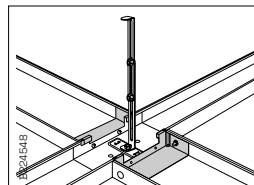
Suspension with End bracket WN17.
